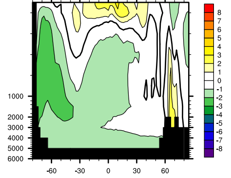
AUSCOM core-Y3 zonal bias
