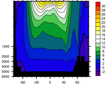
FSU-HYCOM zonal bias
