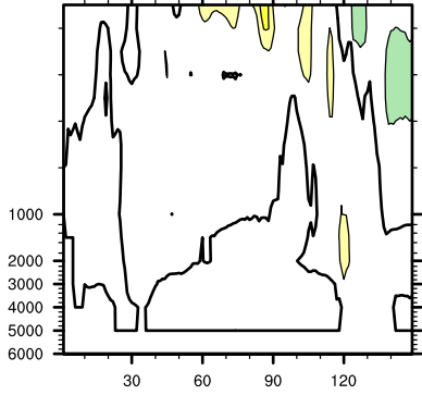
Kie|ORCA zonal bias
