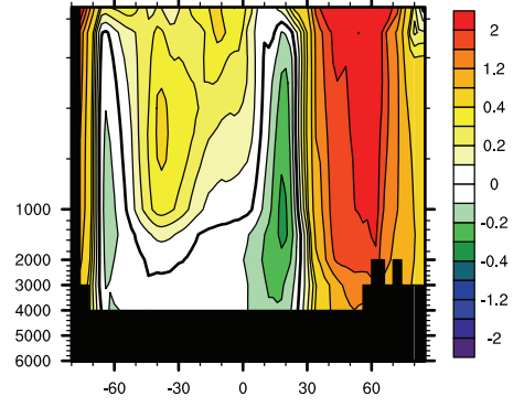
AUSCOM core-X4 zonal bias
