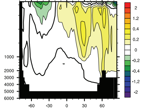
GFDL-HIM zonal bias
