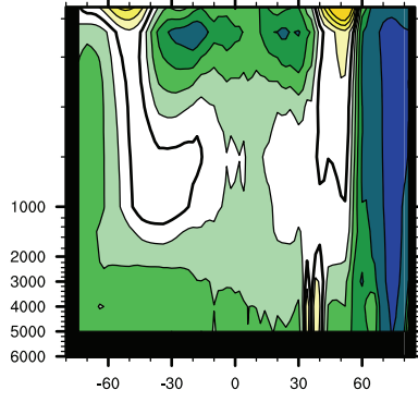
KNMI-MICOM zonal bias
