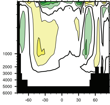
GFDL-MOM zonal bias
