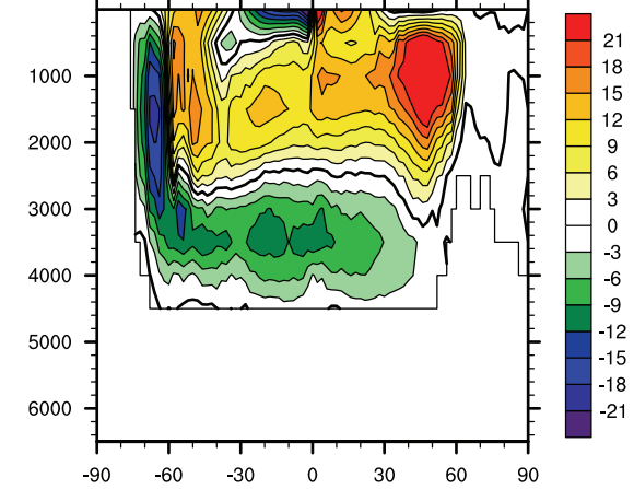
AUSCOM core-X4
