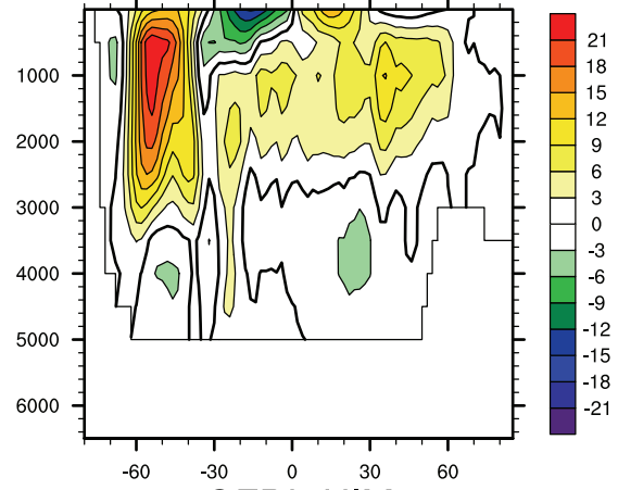
GFDL-HIM
