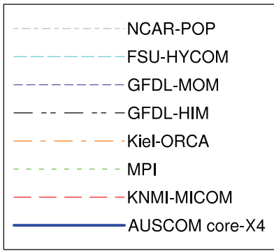
Maximum Atlantic Streamfunction (Sv) at 45°N
