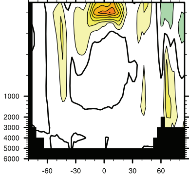
Kie|ORCA zonal bias
