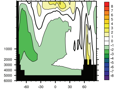
AUSCOM core-Y3 zonal bias
