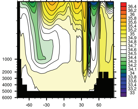
c2_12 zonal bias
