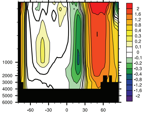
c2_13 zonal bias
