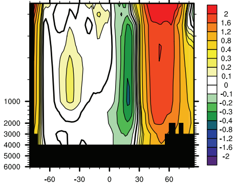
new06 zonal bias
