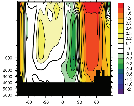
c2_13.1 zonal bias
