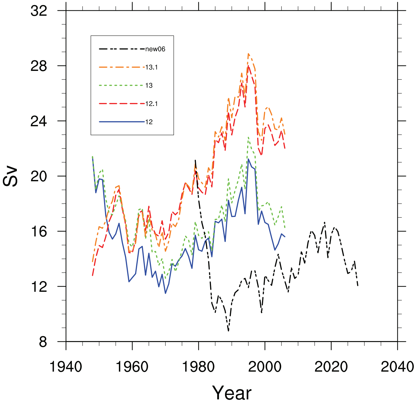
Maximum Atlantic Streamfunction (Sv) at 45°N
